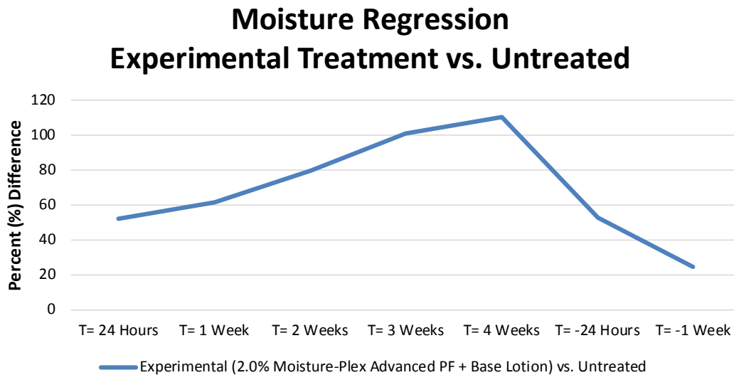
Figure 3. Moisture Regression
