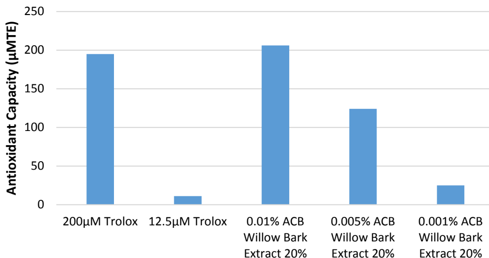
Figure 1. Antioxidant capabilities
