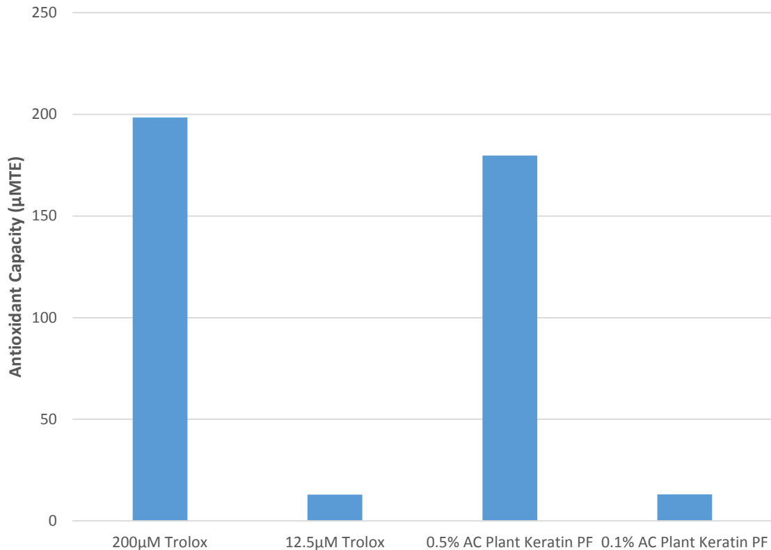
Figure 1. Antioxidant capacities
